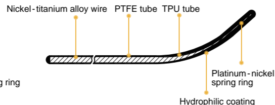
Structure diagram of mixed zebra guide wire
